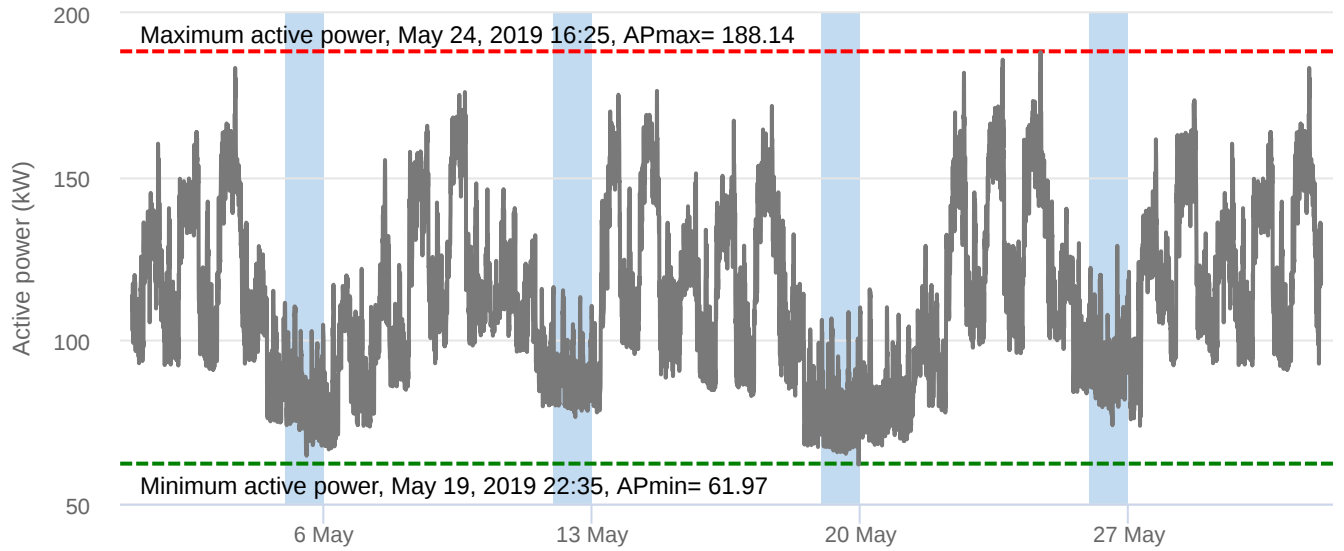
Active power
